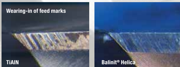
homogeneous wear, no wearing-in of feed marks, high corner stability and shear strength: excellent conditions for multiple regrinding and recoating.
